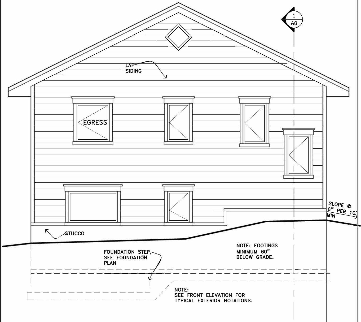
1 NORTH ELEVATION 1/4" = 1'-0"
