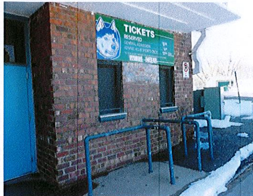
Photo 2: Modify the ticket windows (lower to 36", currently at 43") and modify (or remove) the crowd control railings to provide a 36" wide route (currently 21").
