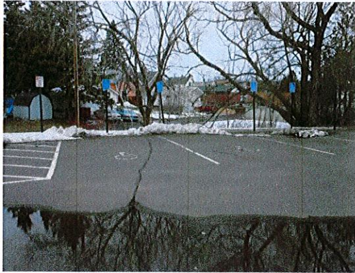
Photo 1: View of accessible parking. Restripe the accessible parking to provide 8' wide aisles (can be shared between 2 spaces).
